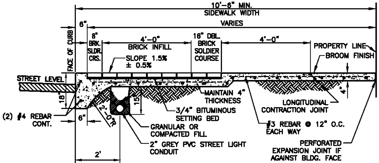
TYPICAL SECTION
