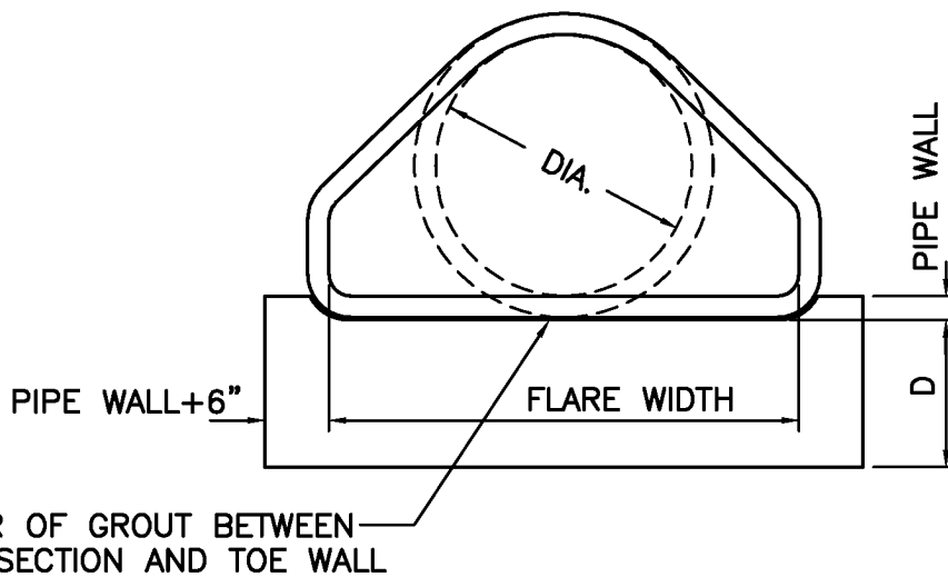
END VIEW
