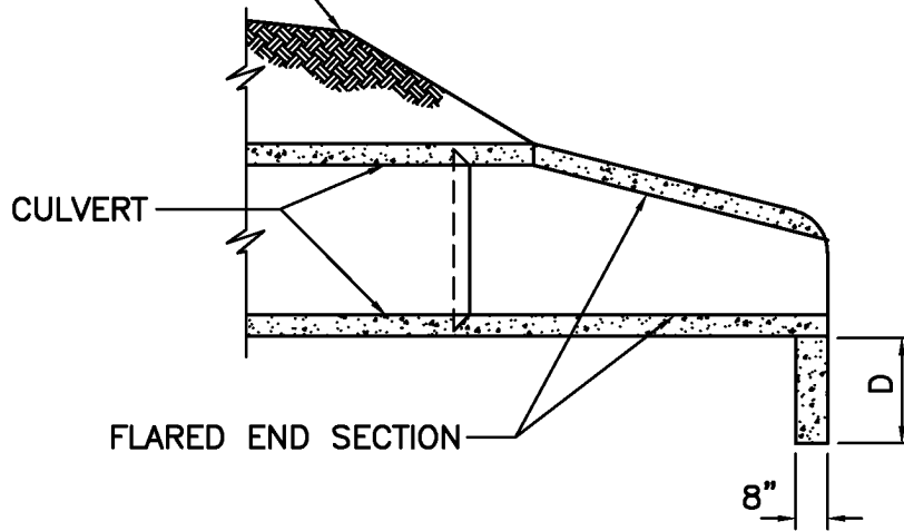
SECTION VIEW
