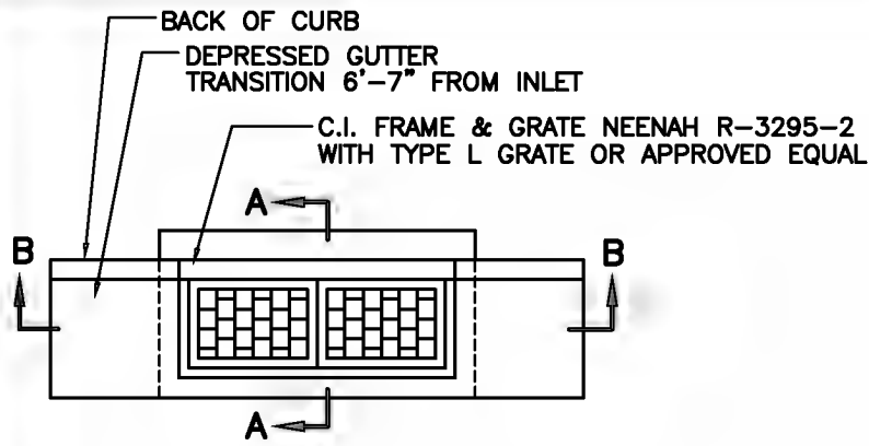
PLAN - DOUBLE
