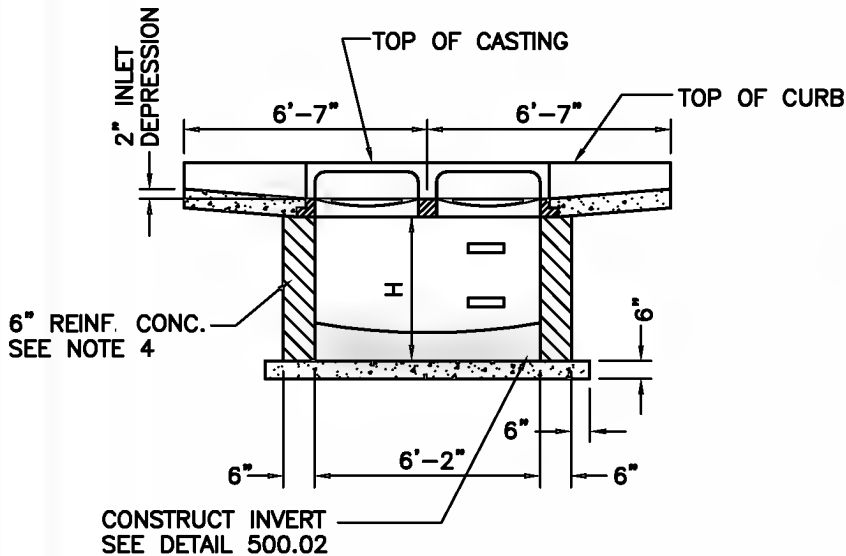
SECTION B-B
