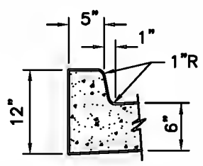
INTEGRAL CURB SECTION
