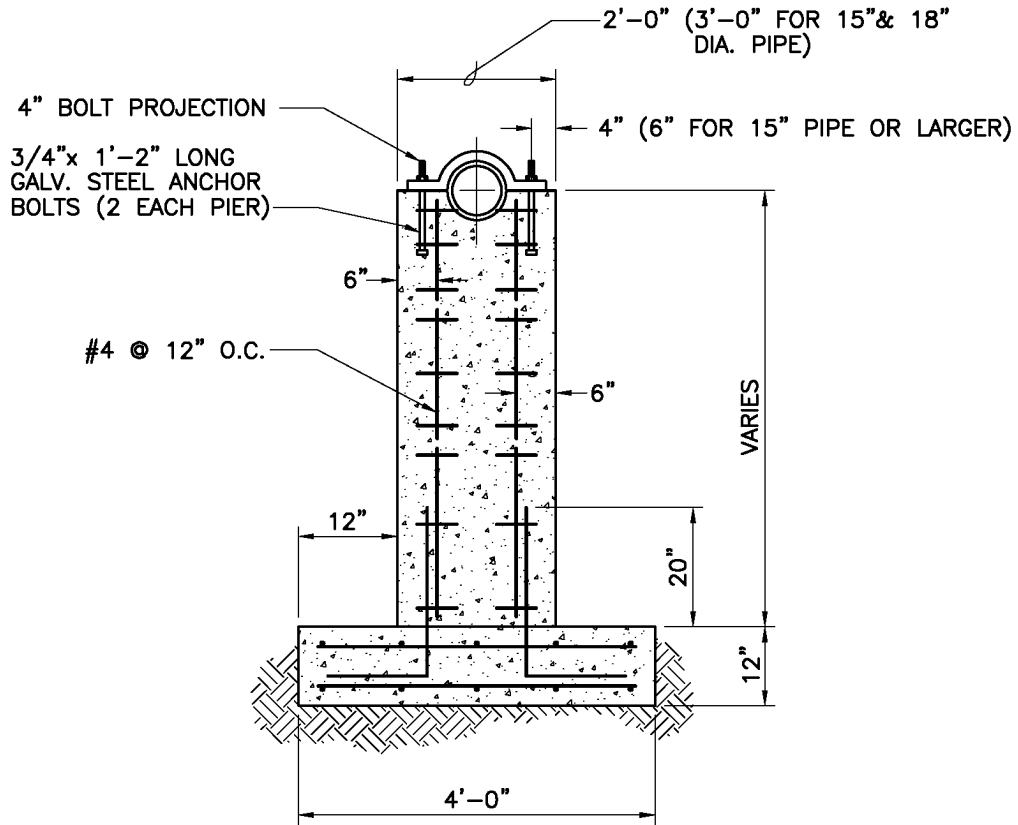
FRONT ELEVATION
