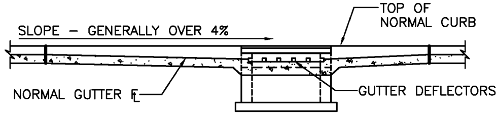
SECTION G-G
