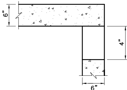
OPENINGS OF 4"
