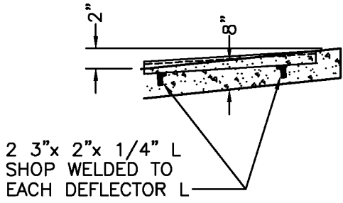
SECTION F-F
