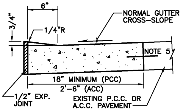
RESIDENTIAL DRIVEWAY CURB MINIMUM RISE
